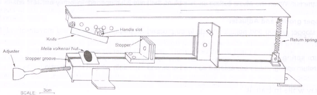
Fig. 1. Melia volkensii seed extractor
