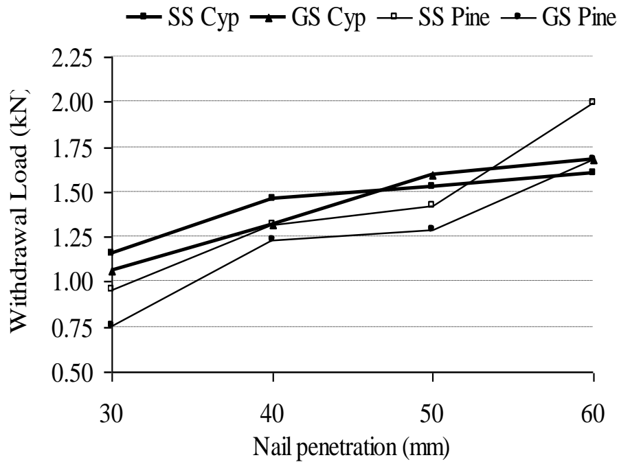
Figure 2. Influence of penetration and wood grade on withdrawal strength
