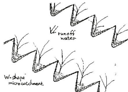
Fig. 5: An arrangement of W-shape MC
