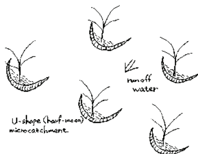
Fig. 4: An arrangement of U-shape MC
